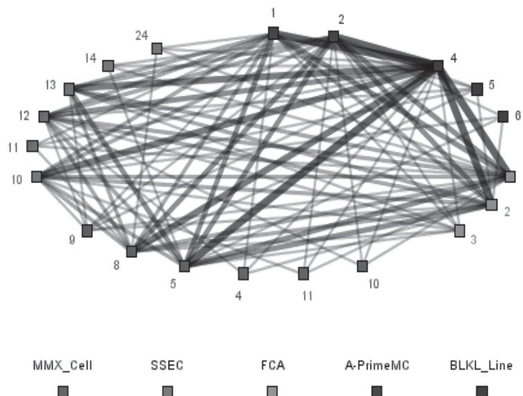
Figure 2. Diagram of fail parts association in hard disk drive assembly line
